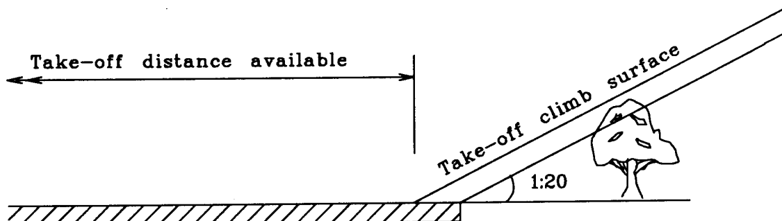
Figure 2. Obstructed design take-off climb surface
