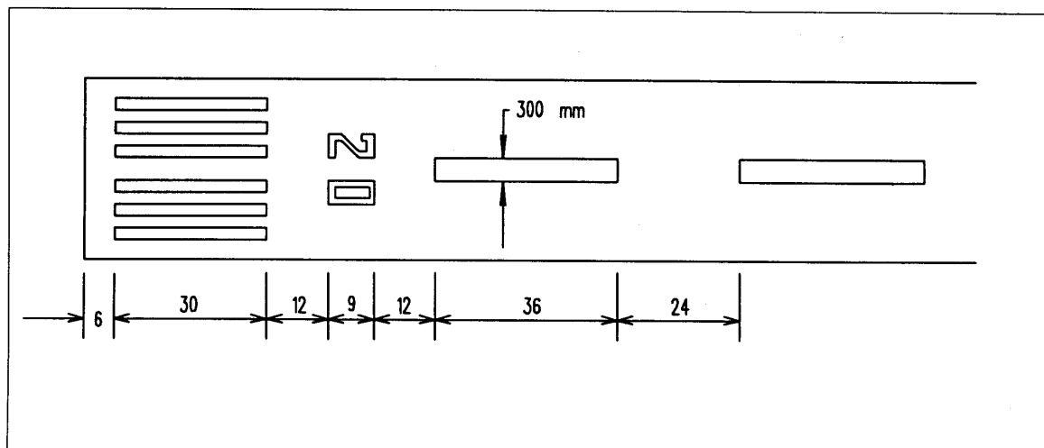
Figure 5-1. Runway markings
